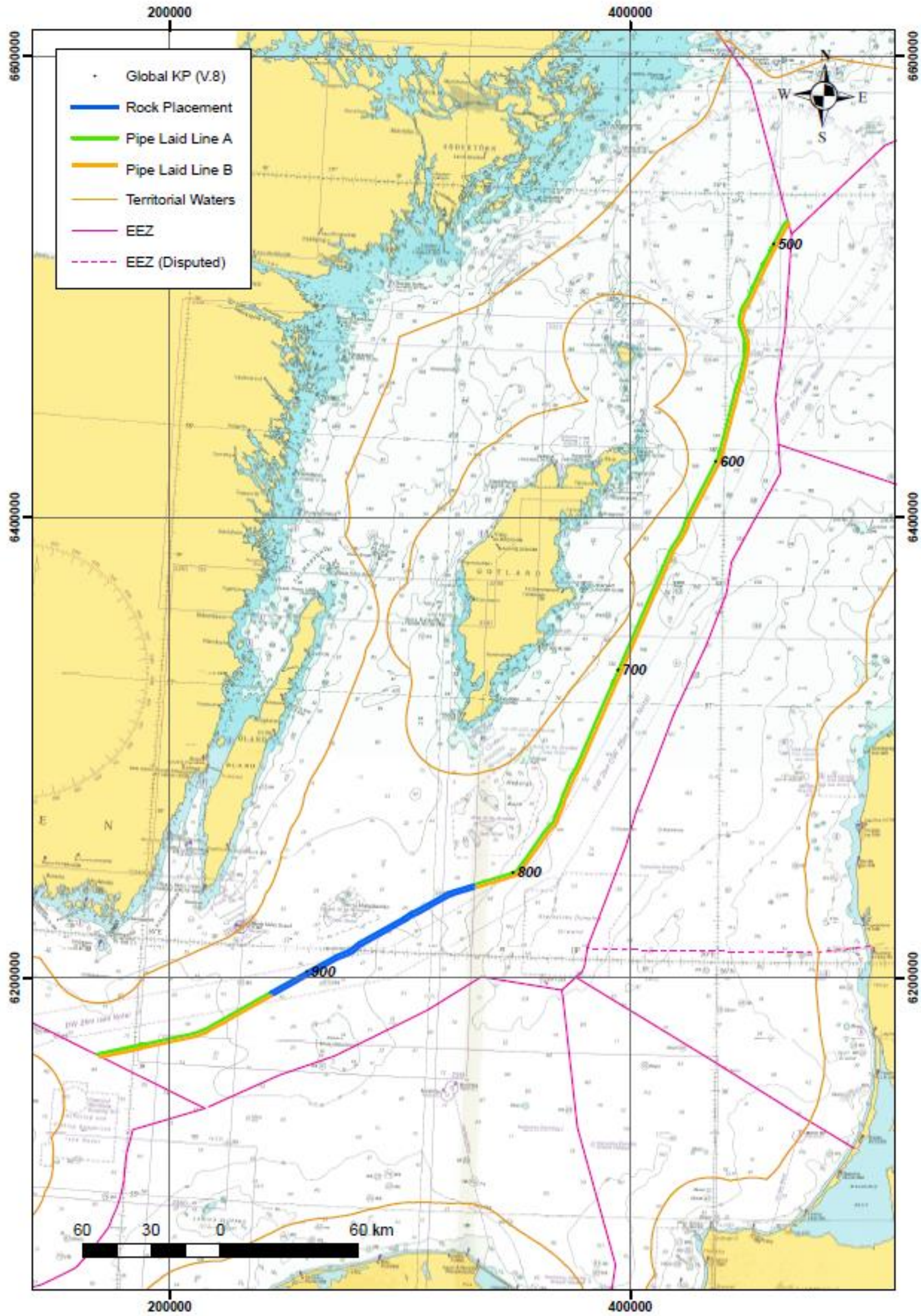
Figure 2: Nord Stream 2 rock placement activities in April in the Swedish EEZ
